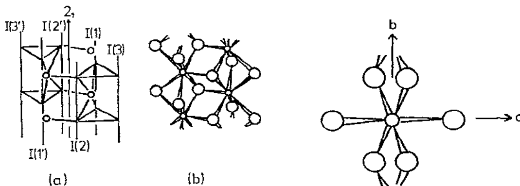
Fig. 7. The coordination of \text{Sn(II)} in \text{SnI}_2 (trigonal prismatic sites). (Reproduced by permission from ref. 24.)
