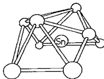
Fig. 25. Projection of the structure of (2-aminobenzothiazolato)nitratotin(II). (Reproduced by permission of the Chem. Soc.)
