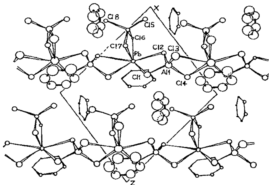
Fig. 50. Chain structure of (C_6H_6)Pb(AlCl_4)_2 \cdot C_6H_6 . (Reproduced by permission of the Am. Chem. Soc.)
