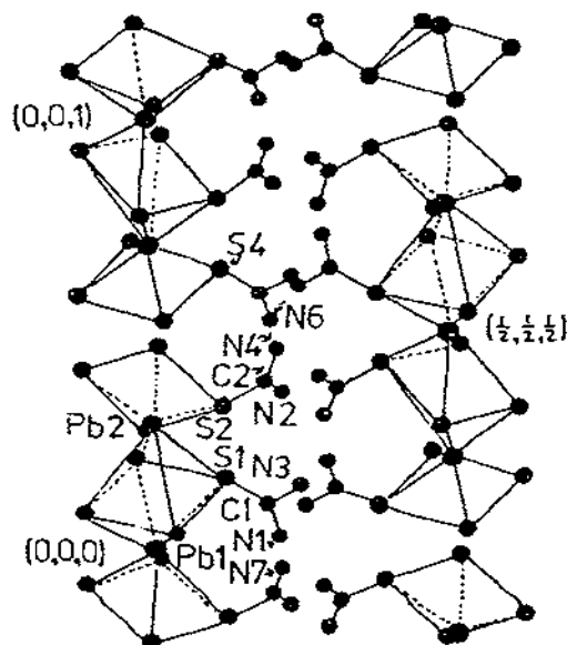
Fig. 41. Structure of \text{Pb}(\text{HCO}_2)_2 \cdot 2 \text{SC}(\text{NH}_2)_2 \cdot \text{H}_2\text{O} . (Reproduced with permission from ref. 161.)
