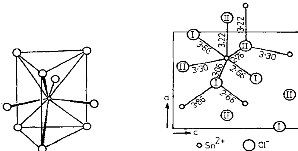
Fig. 3. Coordination of the metal in the \text{PbCl}_2 -type lattice.
