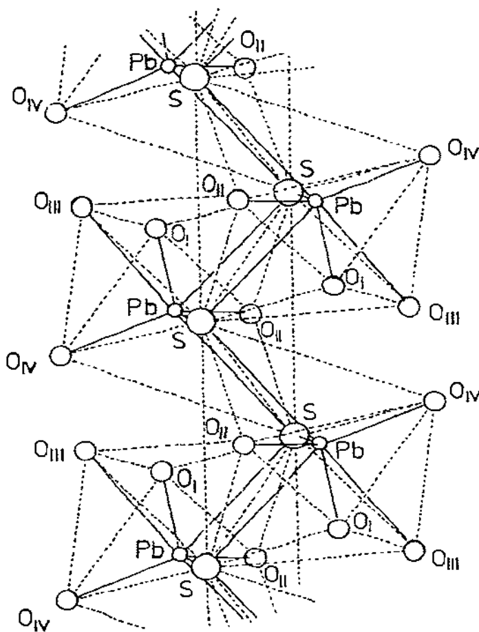
Fig. 43. Clinographic projection of a double chain of coordination polyhedra in mono-thiourea-lead acetate. (Reproduced with permission from Acta Cryst.)
