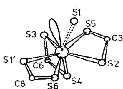
Fig. 37. Coordination around the lead atom in tetraethylammonium tris(ethylxanthato)-lead(II). (Reproduced by permission of Pergamon Press.)
