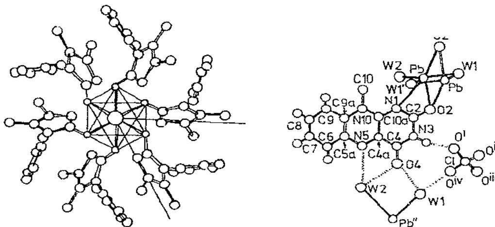
Fig. 33. Coordination of the lead cations in lead hexa-antipyrine perchlorate. (Reproduced by permission from ref. 144.)
